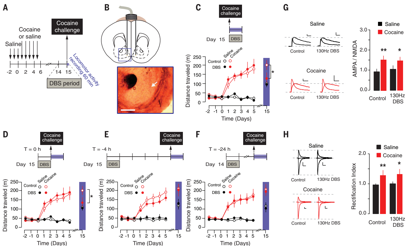
Fig. 1. Classical DBS transiently suppresses locomotor sensitization to cocaine and fails to depotentiate excitatory transmission onto DIR MSNs.
