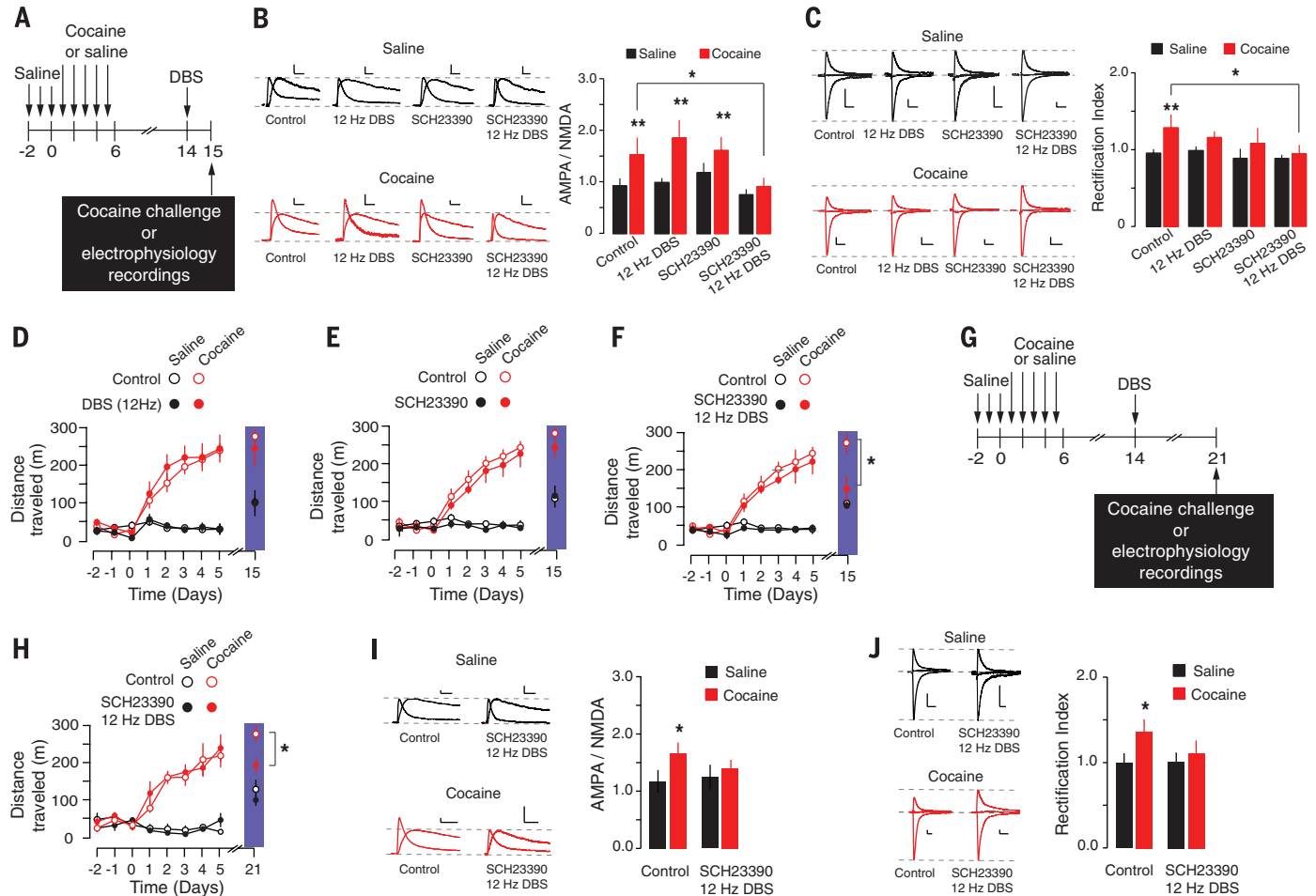
Fig. 3. Optogenetically inspired DBS reverses locomotor sensitization to cocaine and cocaine-evoked plasticity in DIR MSNs. (A) Schematic of experiment. (B) Representative traces and summary plot of AMPA/NMDA ( n = 6 to 8 cells per condition). There was a significant effect of cocaine (ANOVA, cocaine effect F_1 = 10.76 , P = 0.002 ) and a significant interaction between DBS and SCH23390 treatment ( F_1 = 5.74 , P = 0.020 ) on the AMPA/NMDA ratio. AMPA/NMDA in cocaine-treated animals treated with DBS was reduced to the level of that in saline-treated controls (cocaine control versus cocaine + DBS, t = 2.39 , P = 0.029 ). Sample traces are of AMPA and NMDA EPSCs at +40 mV from saline- (black) and cocaine-treated (red) animals. (C) Representative traces and summary plot of rectification index ( n = 6 to 8 cells per condition). There was a significant effect of cocaine on RI (ANOVA, cocaine effect F_1 = 6.04 , P = 0.018 ); cocaine-treated animals that had undergone DBS were not different from saline-treated controls (cocaine control versus cocaine + DBS, t = 2.16 , P = 0.046 ). Sample traces are of AMPAR EPSCs at -70, 0, and +40 mV from saline- (black) and cocaine-treated (red) animals. (D) 12-Hz DBS alone (controls: saline/cocaine = 9/10, 12-Hz DBS: saline/cocaine = 6/8) or (E) SCH23390 alone (controls: saline/cocaine = 9/9; SCH23390: saline/cocaine = 5/7) did not affect sensitization to cocaine. (F) 12-Hz DBS in combination with SCH23390 reduced the sensitized locomotor response to cocaine (controls: saline/cocaine = 9/10;
